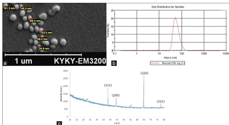
Figure 4: Characterization of Ag nanoparticles. (a): SEM image of synthesized silver nanoparticles by fruit extract of Vitex agnus castus L; (b): DLS analysis showing diameter of synthesized silver nanoparticles by fruit extract of Vitex agnus castus L; (c): X-ray diffraction patterns (XRD) of biosynthesized silver nanoparticles
